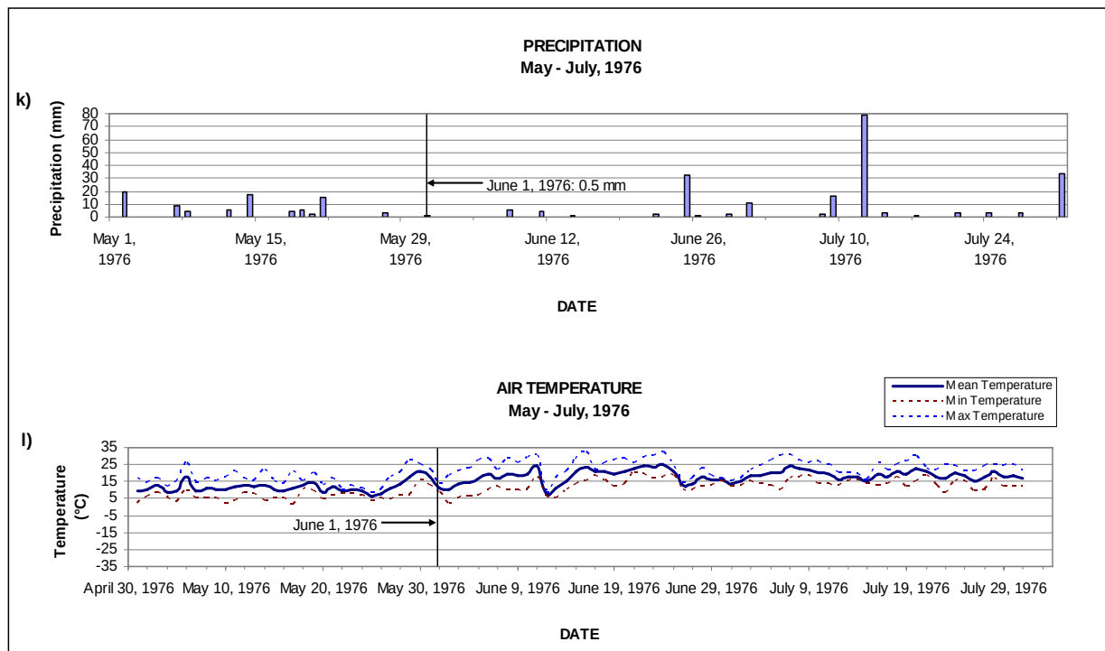
k) Precipitation from May 1st - July 31st, 1976. l) Air temperature from May 1st - July 31st, 1976.
