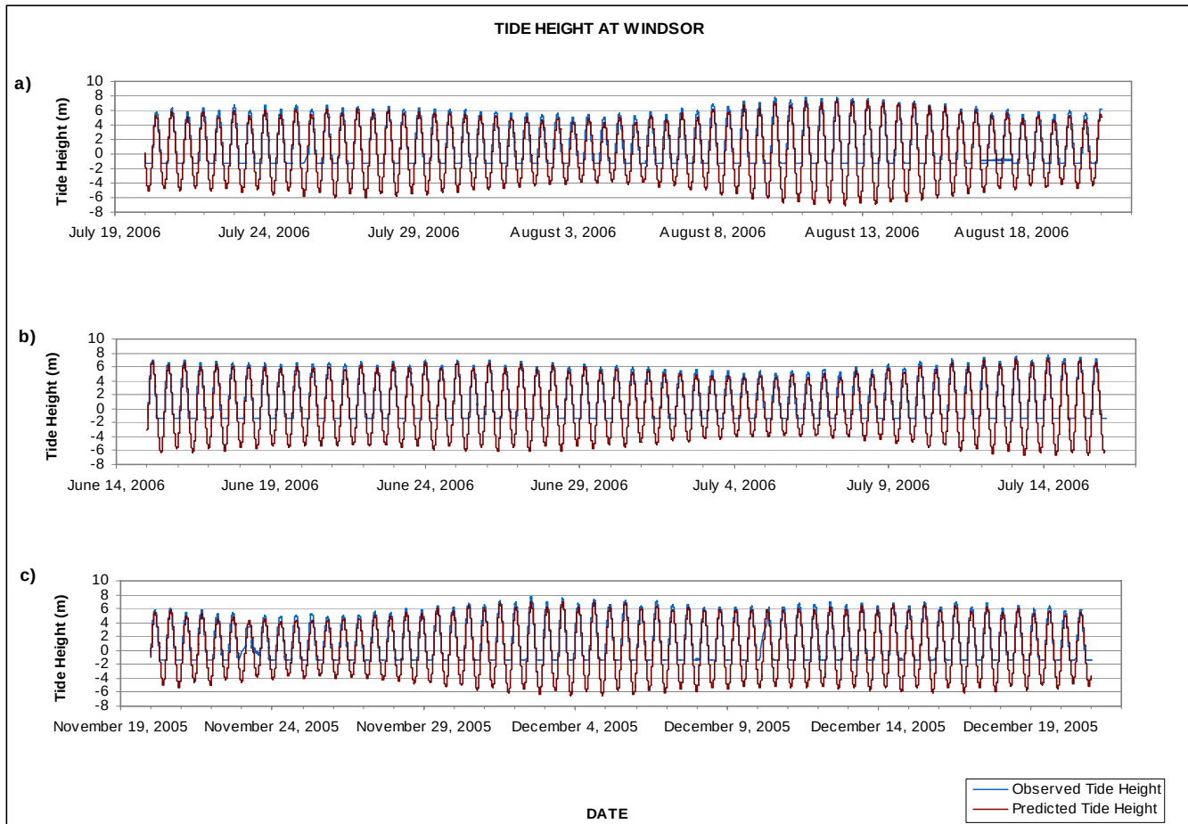
Figure A.3: Graphs of observed tide height and predicted tide height. Observed tide height was recorded at the Weatherhawk tm meteorological station (44.99 N, -64.15 W), and predicted tide height was obtained using Tides and Weather tm software
