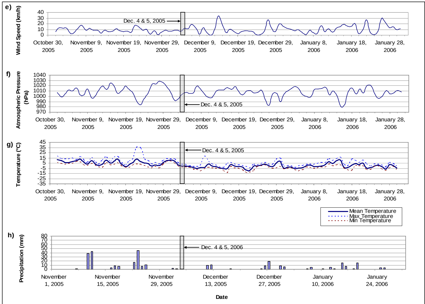
e) Mean daily wind speed from November 1st 2005 – January 31 st , 2006. f) Mean daily atmospheric pressure from November 1st 2005 – January 31 st , 2006. g) Mean daily temperature, minimum temperature, and maximum temperature from November 1st 2005 – January 31 st , 2006. h) Total daily precipitation from November 1st 2005 – January 31 st , 2006.
