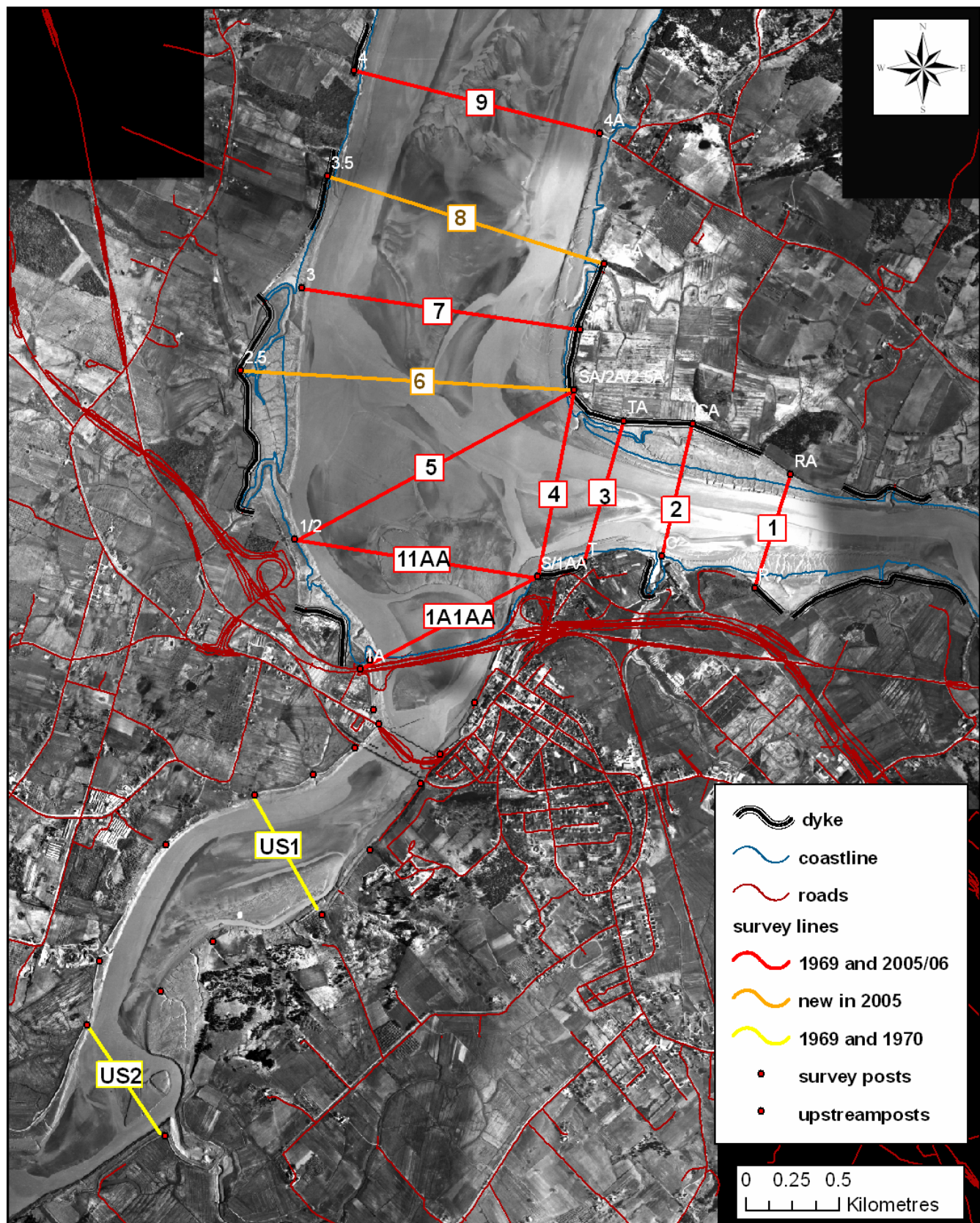
Figure 3.2 a) Location of historical and contemporary survey lines closest to the Windsor causeway. Although additional upstream surveys were conducted as indicated by the survey posts, those data were only collected in Nov 1970, after the causeway was completed and no comparable data are available. Note the road and coast vector layers are based on data from 1986 to 1996 (Service NS Municipal Relations) overlain onto a 1964 digital photo mosaic.
