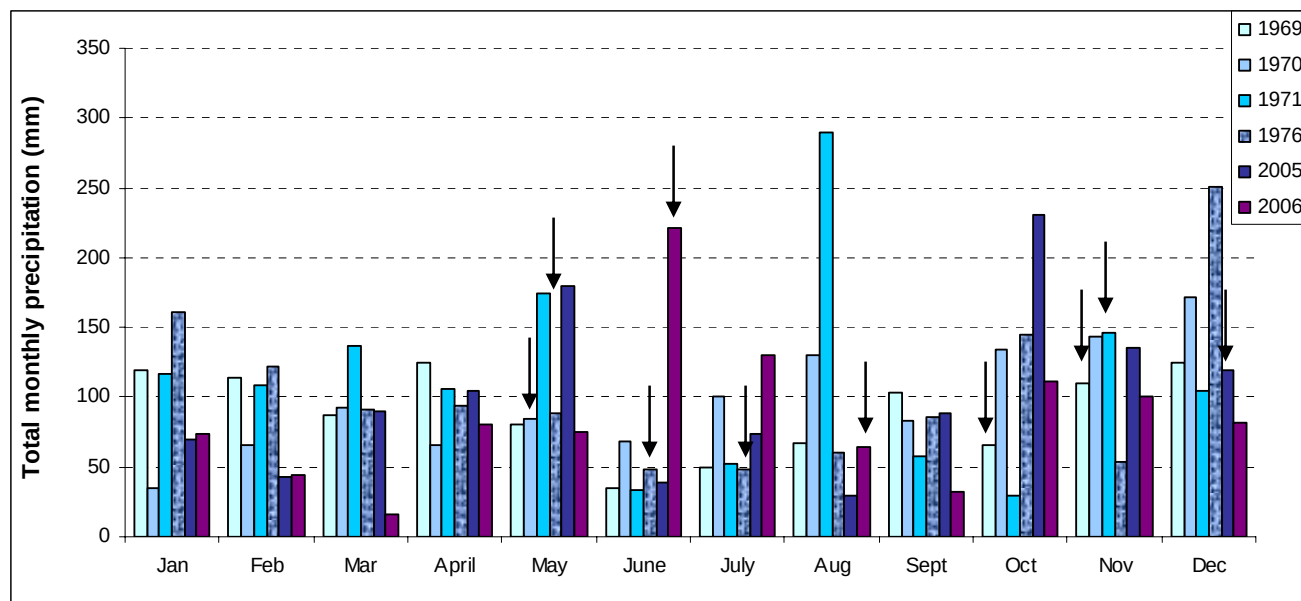
Figure 3.4: Total monthly precipitation at Kentville (45.07 N, -64.43 W). Months during which surveys were conducted indicated by an arrow.
