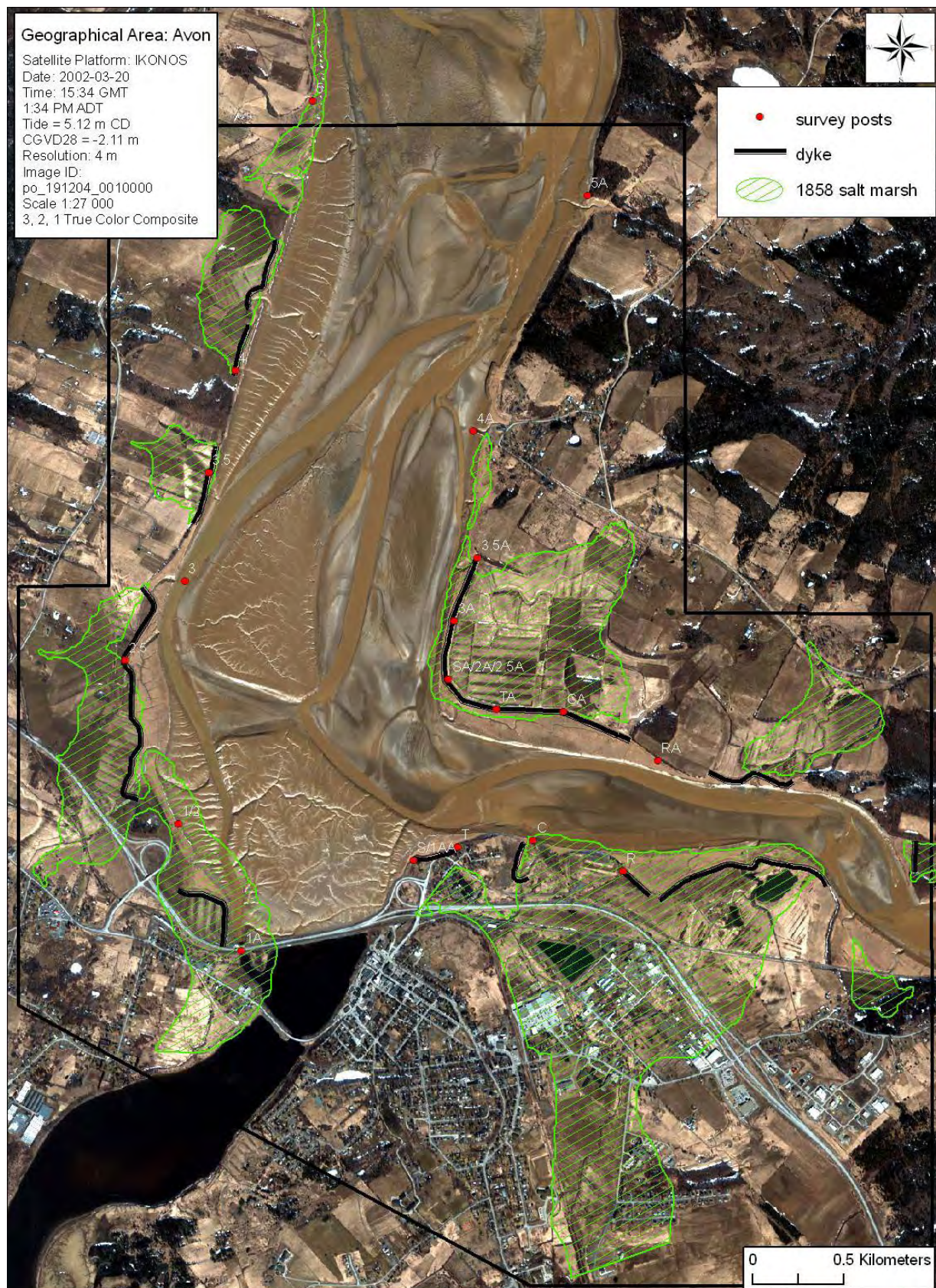
Figure 4.20: Multispectral IKONOS satellite image illustrating position of main channels and intertidal bedforms on March 20, 2002. Resolution of satellite is 4 m. Location of 1858 marsh provided for reference. No vegetation is visible on Windsor mudflat/salt marsh since it is too early in the growing season and most of the previous year's growth would be dead and/or sheared off therefore would not contain chlorophyll which could be detected by the satellite.
