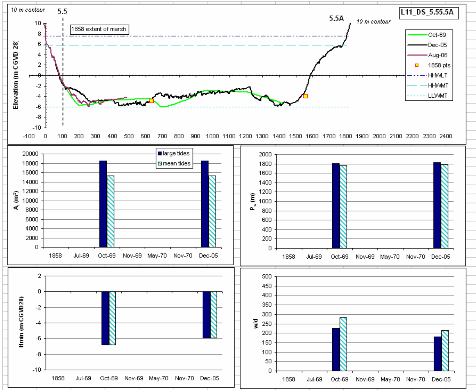
Figure 4.30: Cross sectional profile for Line11_DS_5.55.5A and associated hydraulic geometry parameters on the Avon River. Note change in vertical exaggeration on cross sectional profiles to 125 X. Distance on cross sectional profile in metres.
